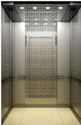
SG-K12 选配Optional 吊顶：镜面顶板、筒灯 轿壁：镜面蚀刻与发纹不锈钢组合 扶手：发纹不锈钢扶手 地板：PVC（可选大理石） Ceiling: Mirror stainless steel, LED light Car wall:Mirror etching+hairline stainless steel Handrail: hairline stainless steel tube Floor:PVC(optional marble)
